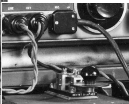
Key and Plug Assembly No. 2B used with No. 12 Set and R107 fitted in Truck 15-cwt, 4-wheeled Wireless. The enlarged section (above) of this photo shows the key and base plate fitted in the slide.
