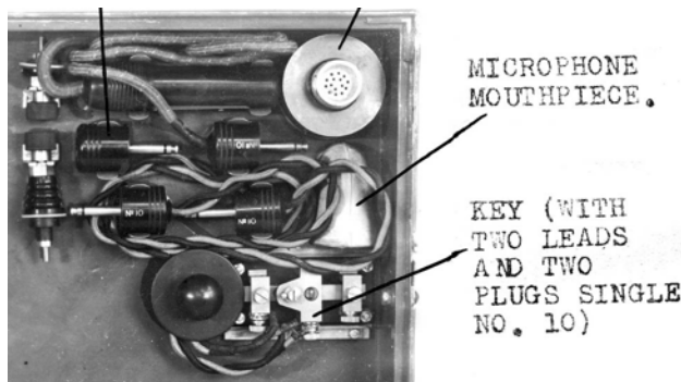
Interior view of No. 2 Set sender lid (above). The Key and Plug Assembly No. 1 or 2 (with a Key W.T. 8 Amp No. 2) was normally stowed in this position when not required.
