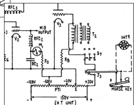
Part of circuit diagram Wireless Sender No. 2 showing the keying circuits and connections to the interruptor for I.C.W. keying (above).
