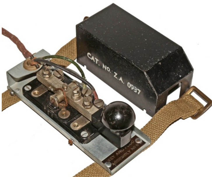
Key and Plug Assembly No. 9 ver. 2 with protective cover opened . The Morse key was a Key W.T. 8 Amp No. 2 Mk.II.
